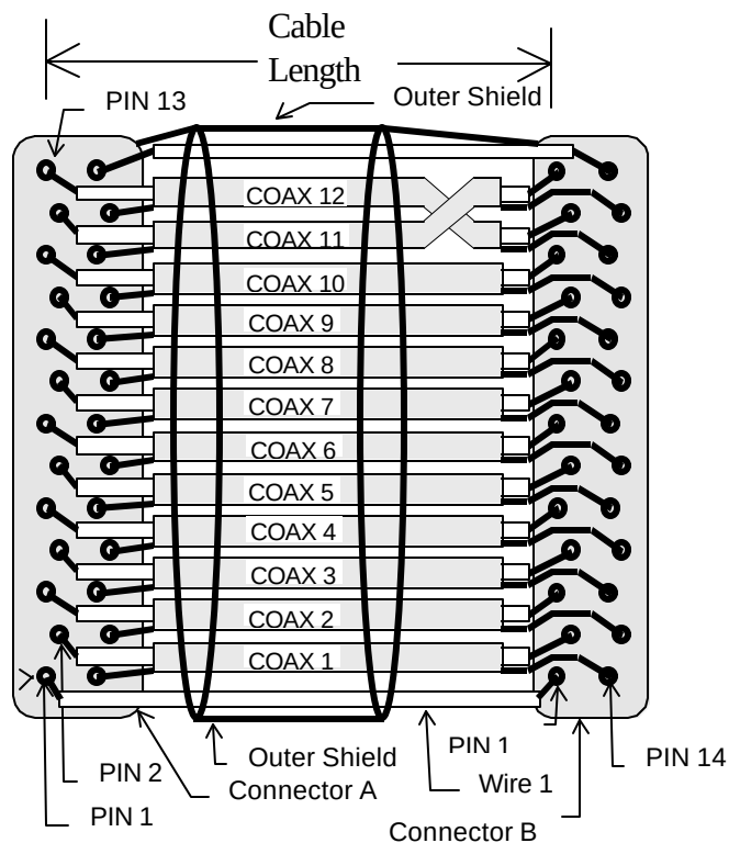
Figure 3. Link port standard cable assembly
