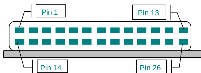
Figure 1. Honda RMCA-26JL-AD connector
